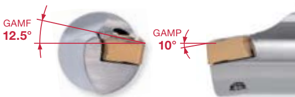
MINIFORCE A12M-SCLXR06-D140
