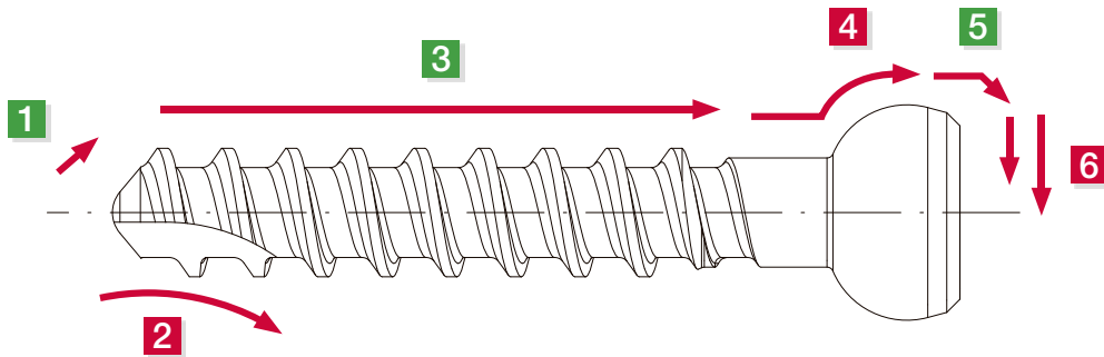
1 Front Turning
